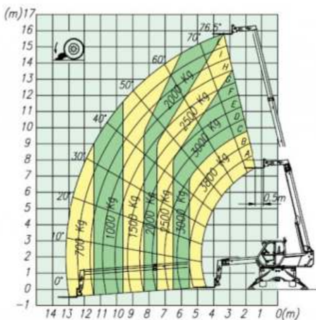
Roto 38.16 S and 38.16 - With forks on stabilisers - Through 415°
