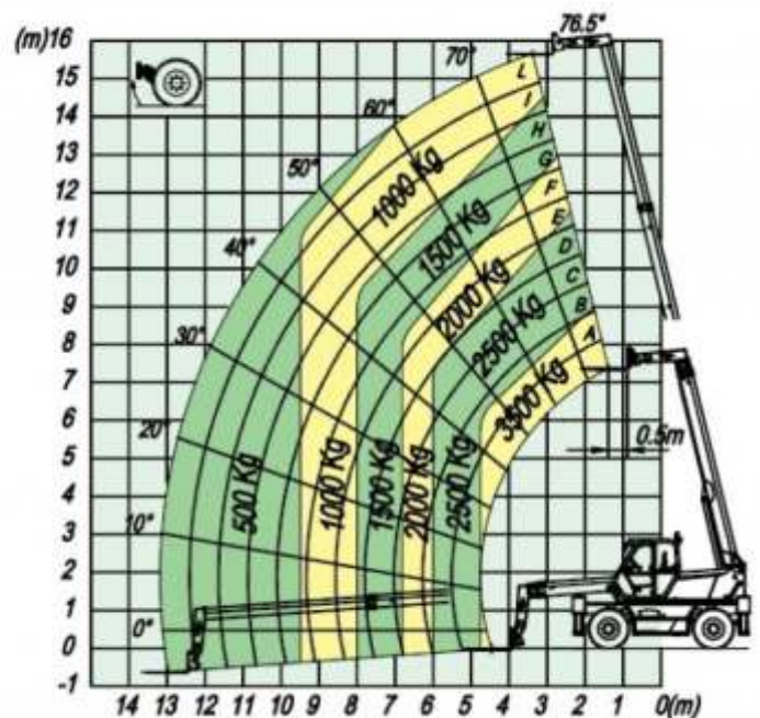
Roto 38.16 S - With forks on tyres - Front
